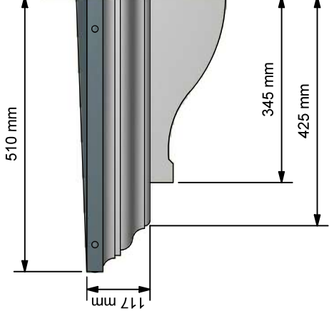
Side View ( 1:10 )
